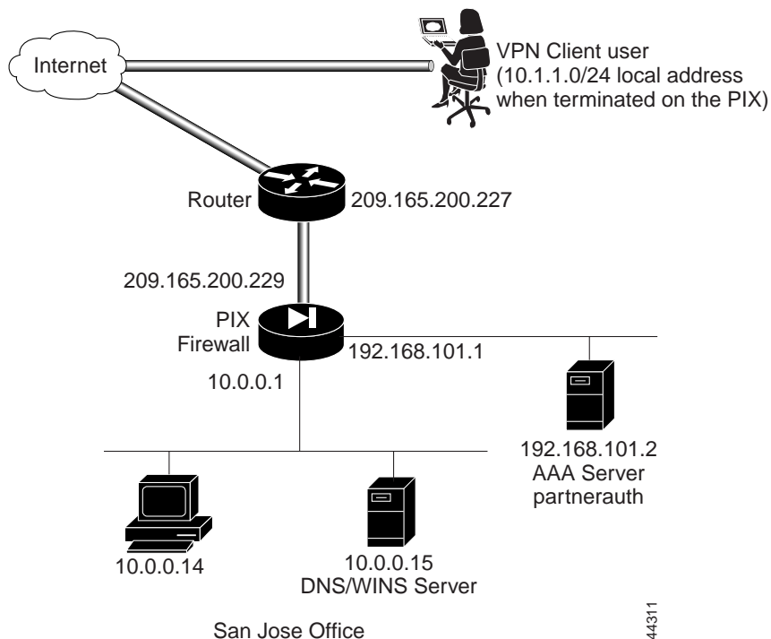
Figure 10-1 VPN Client Access
